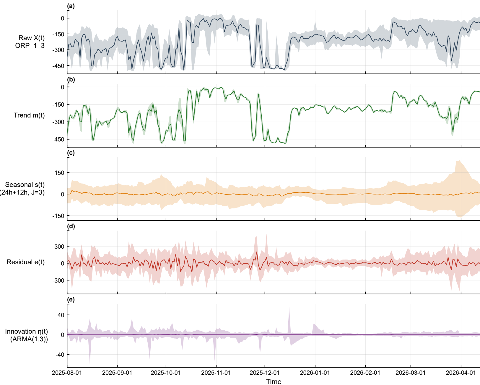
Full-span daily overview — ORP_1_3 (pre_anoxic_rear, min) [2025-08-01~2026-04-13]
